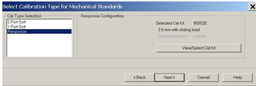
Figure 33 Response
