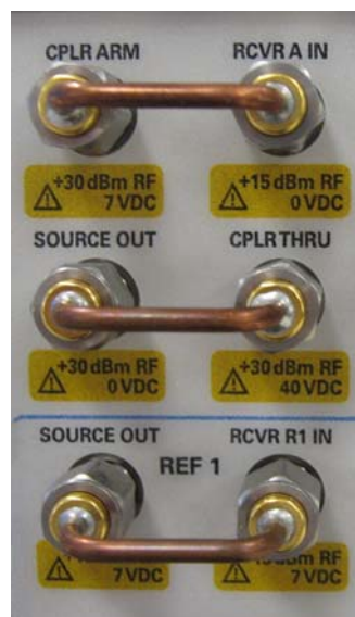
Figure 20 Front Panel Jumpers
