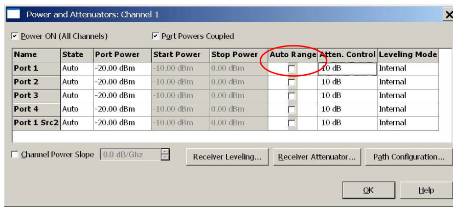
Figure 26 Attenuator Control
