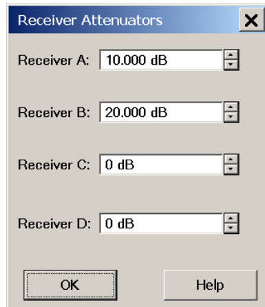
Figure 28 Receiver Attenuators
